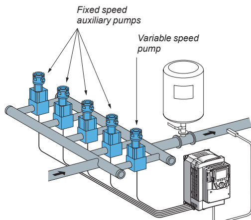
Example of configuration of a pumping system with the VW3 A3 502 multi-pump card
