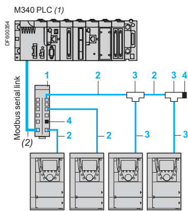
Example of Modbus diagram with connection via splitter box and RJ45 connectors
