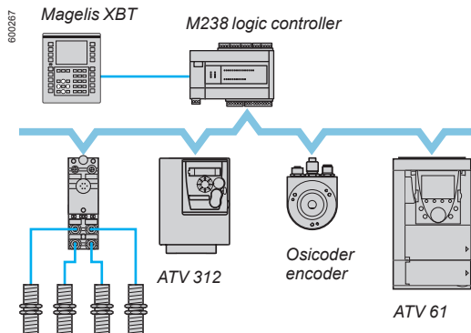
Example of configuration on CANopen machine bus
