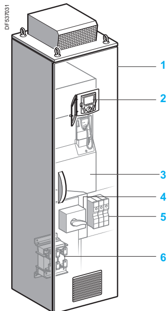
The standard ATV 61EXC offer
