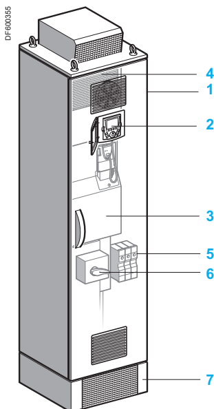
The standard ATV 61EXS5●●●●● offer
