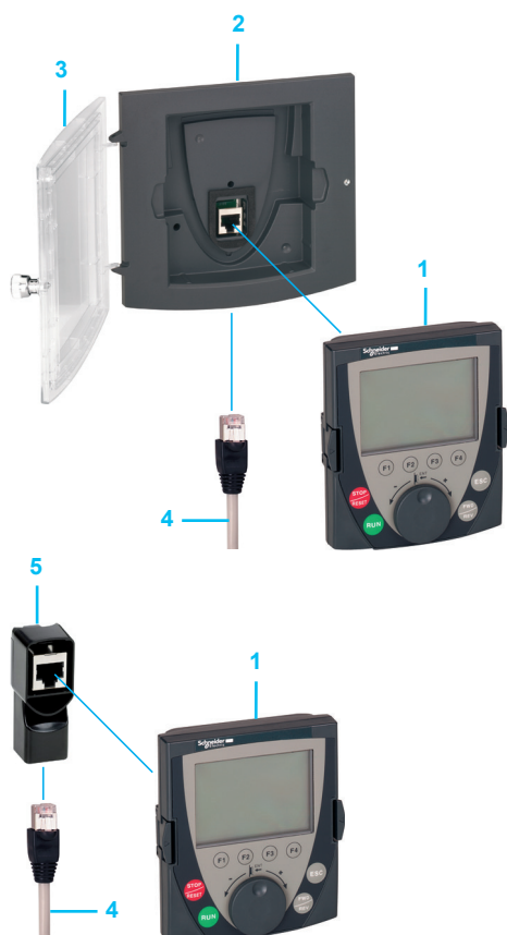
Remote mounting accessories for the graphic display terminal
